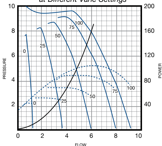
Performance Curves at Different Vane Settings
