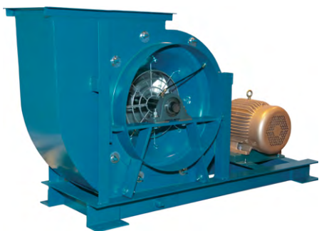
Arrangement 1 fan with optional unitary base, pie-shaped split housing, shaft and V-belt drive guard.
