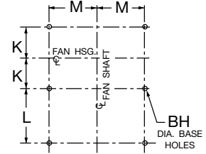
FOUNDATION PLAN
