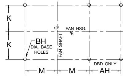
FOUNDATION PLAN
