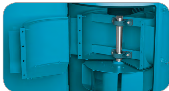
Removable Bearing Cover Plate on Model TSL Clamshell
